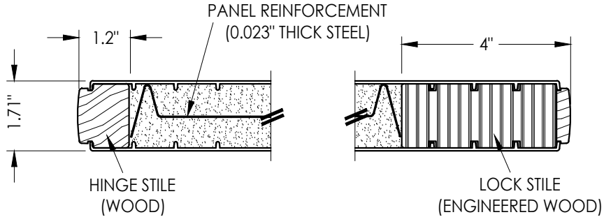
3/4 HORIZONTAL CROSS SECTION
