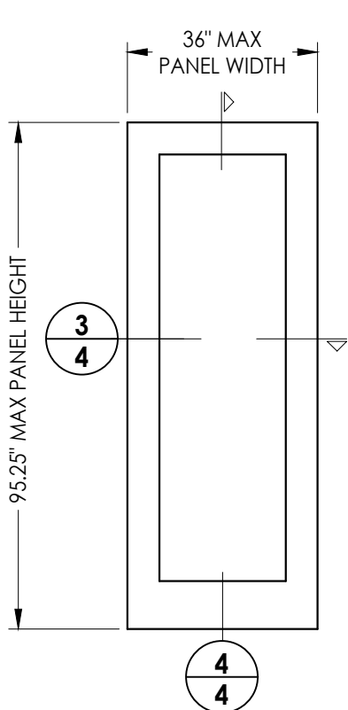
3/4 FIBERGLASS DOOR/SIDELITE PANEL Therma-Tru 8'-0" (Wood Edge)
