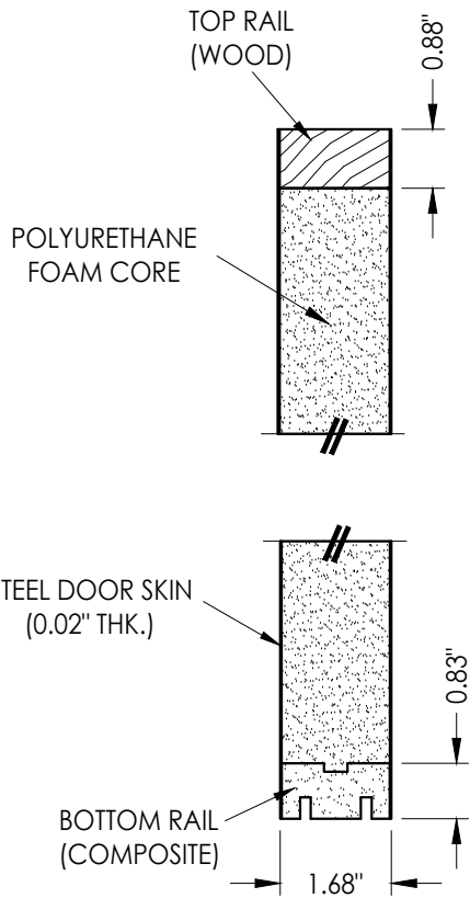
2 5 VERTICAL CROSS SECTION
