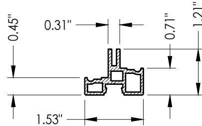
2A INTERIOR FRAME 1-1/4" GLAZING
