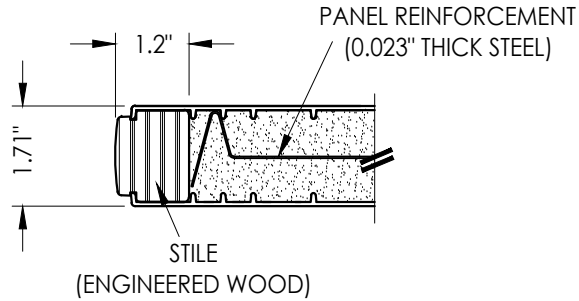
1/4 HORIZONTAL CROSS SECTION
