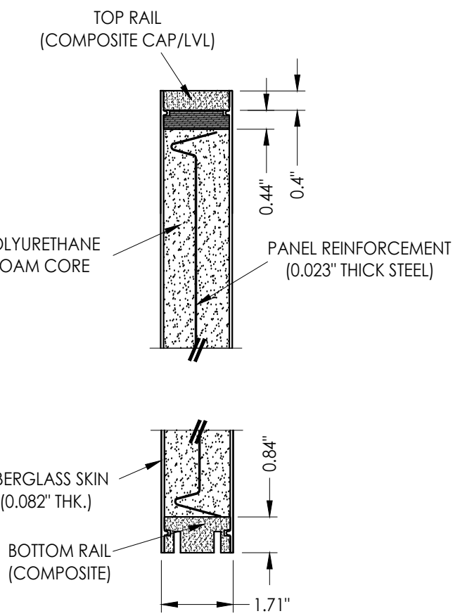
4 3 VERTICAL CROSS SECTION
