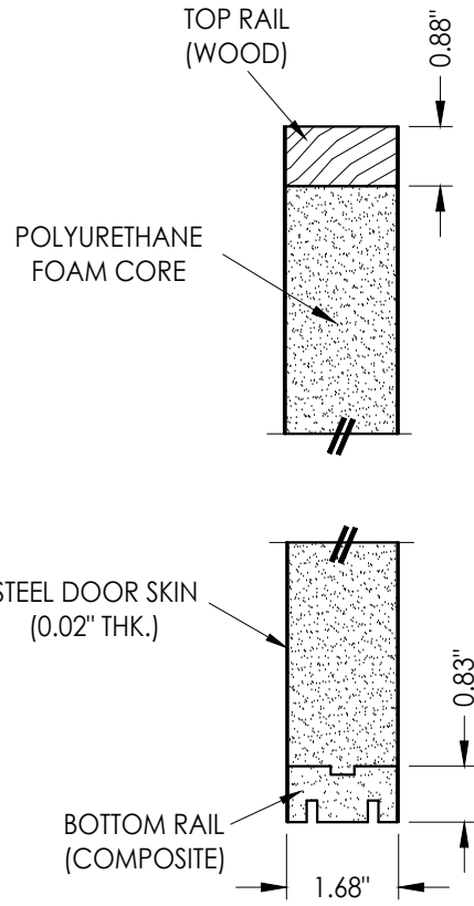
4 5 VERTICAL CROSS SECTION
