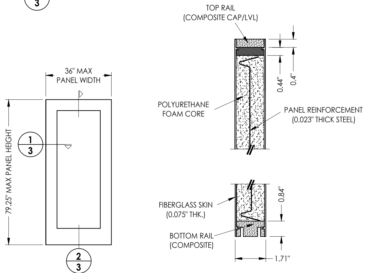
FIBERGLASS DOOR/SIDELITE PANEL Therma-Tru 6'-8" (Composite Edge)
