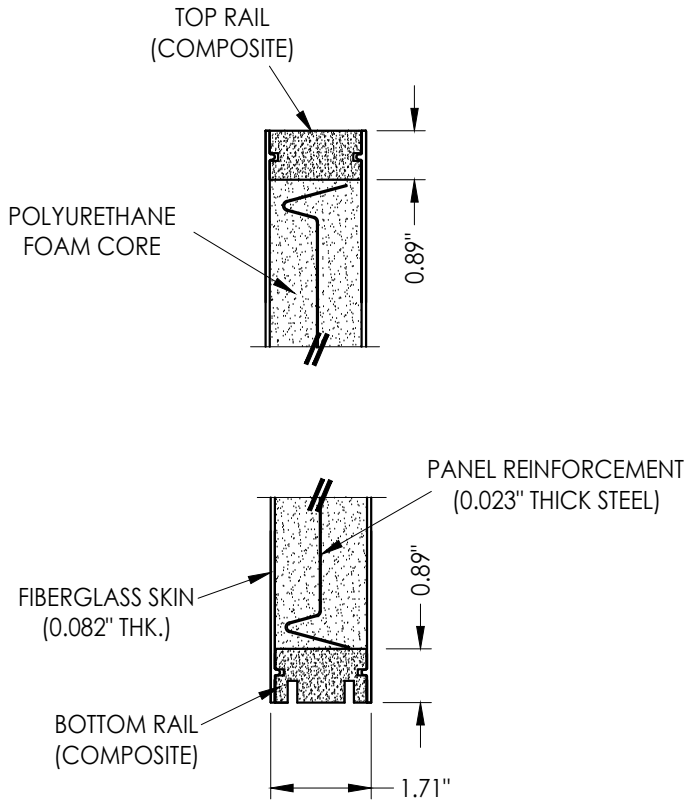
4/4 VERTICAL CROSS SECTION
