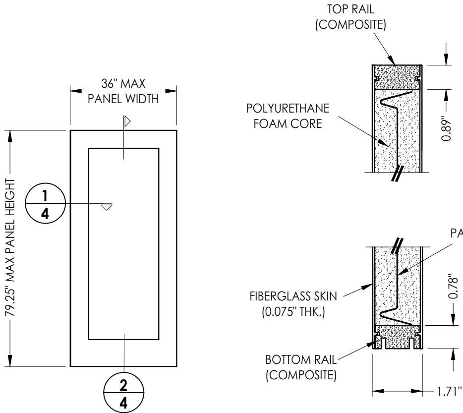
2/4 FIBERGLASS DOOR/SIDELITE PANEL Therma-Tru 6'-8" (Wood Edge)
