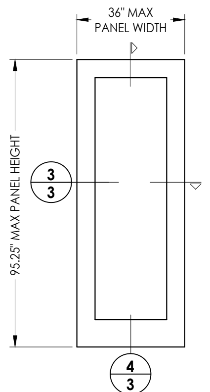
FIBERGLASS DOOR/SIDELITE PANEL Therma-Tru 8'-0" (Composite Edge)
